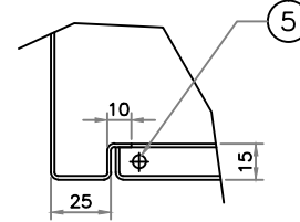
DETAIL X
