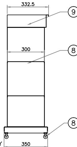
DETAIL X
